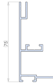
75mm Fabric-lite section
